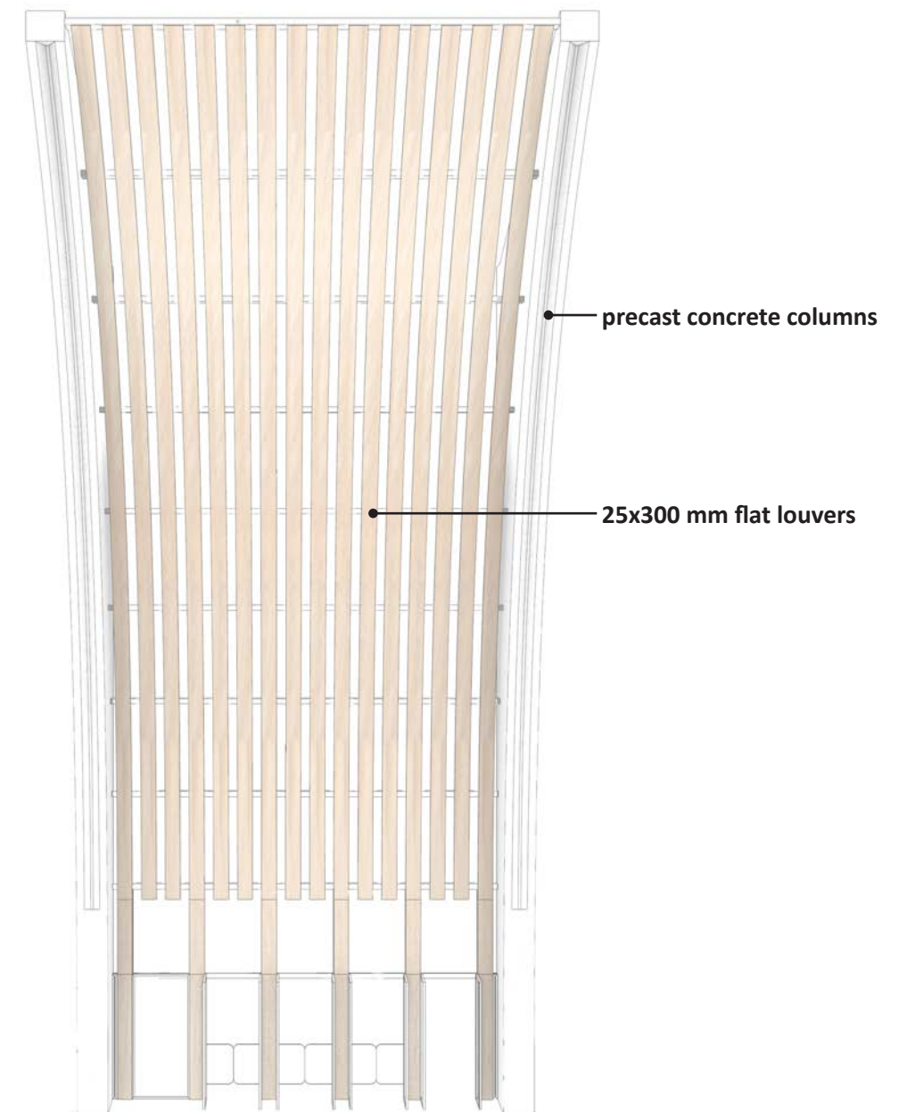
OPTION 2 - CURVED TIMBER LOUVERS - READY AVAILABLE SECTIONS
