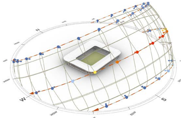
SUNPATH DIAGRAM
