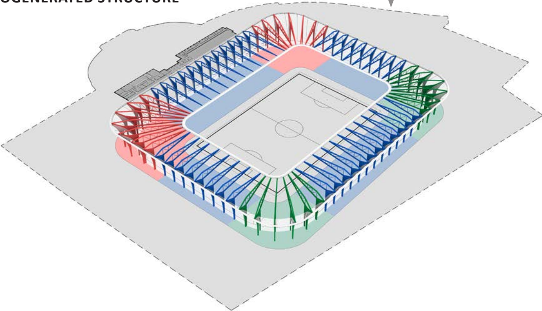
AUTOGENERATED STRUCTURE
