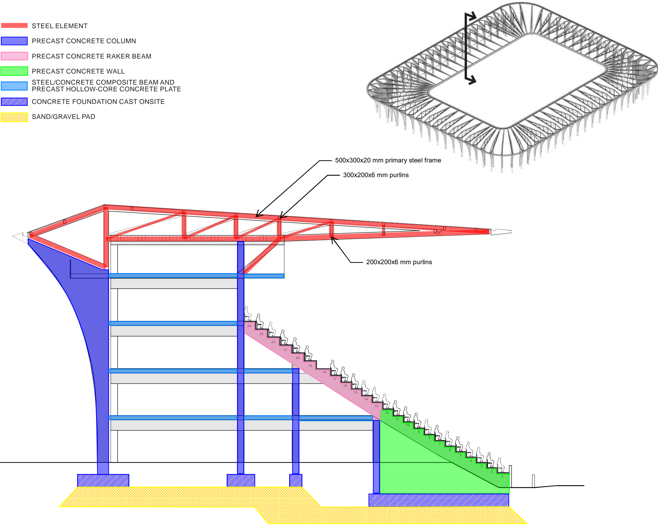
MAIN STRUCTURE - SECTION OF MAIN STAND AND BUILDING
