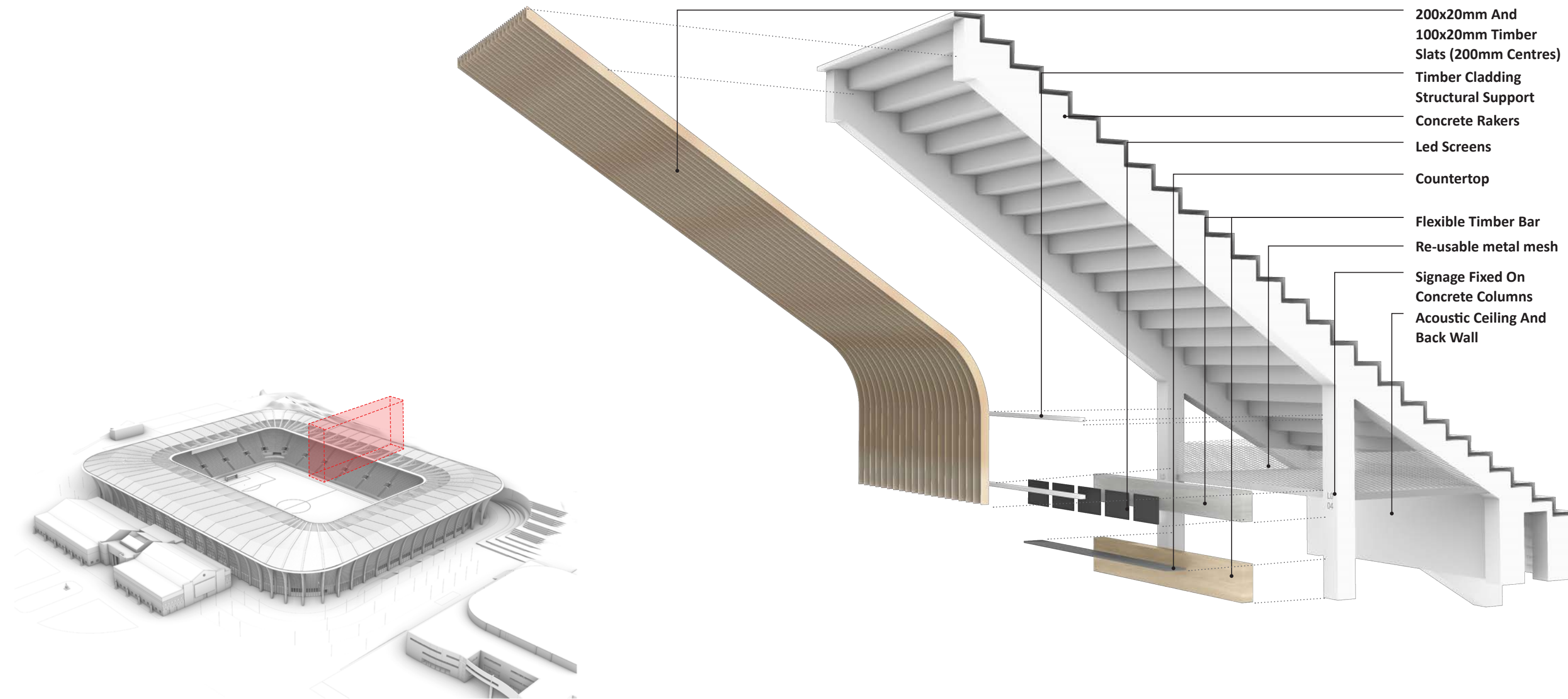
EXPLODED AXONOMETRIC
