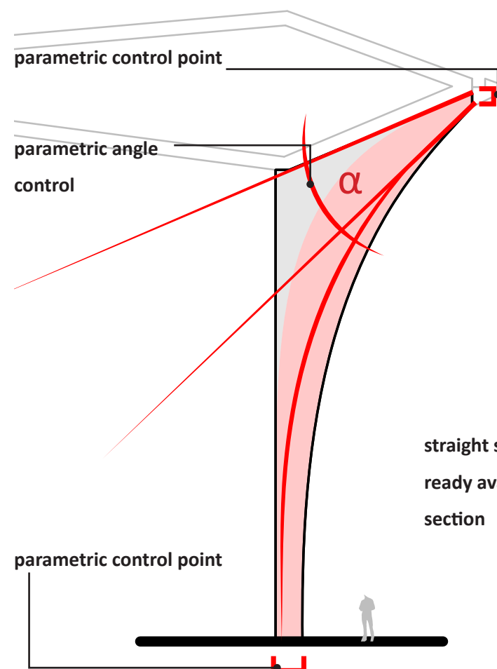
TYPICAL BAY
